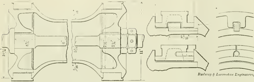
PISTON VALVE.—MISSOURI PACIFIC RAILWAY.
